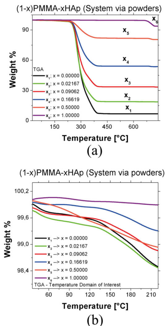
Figure 2. TGA heating profiles for x_i ( i=1-6 ) concentrations of the (1-x)PMMA-xHAp system via powders to determine system's mass loss (a) among 35 – 751 °C (b) in TOI among 45 – 210 °C approximately.
