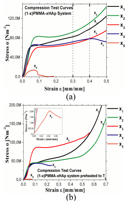
Figure 6. Compression profiles for the mechanical assay on the blocks with x_i ( i=1-5 ) concentrations of the (1-x)PMMA-xHAp binary system, where (a) PMMA+HAp polymerized system without thermal treatment with a fracture domain at 0.30 – 0.42 % compression strain; and (b) PMMA+HAp polymerized system with thermal treatment of 30 min at T_g glass transition temperature.
