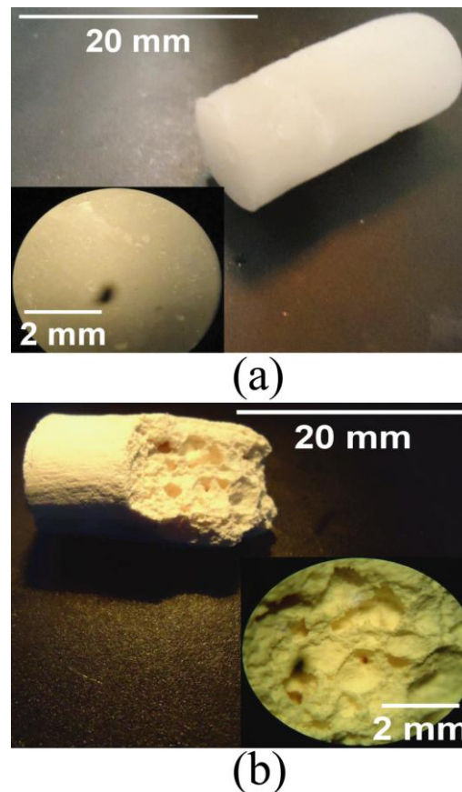
Figure 7. Stereoscopic images of the block surfaces, where (a) to PMMA only or x_1 concentration without thermal treatment; (b) to x_5 concentration parameter with thermal treatment for 30 min at the T_g glass transition temperature.
