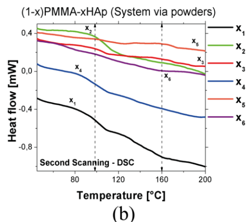
Figure 4. DSC heating curves for the six [x] concentrations of the (1-x)PMMA-xHAp system via powders in TOI between 45 – 200 °C. The Heat Flux is presented in [mW].
