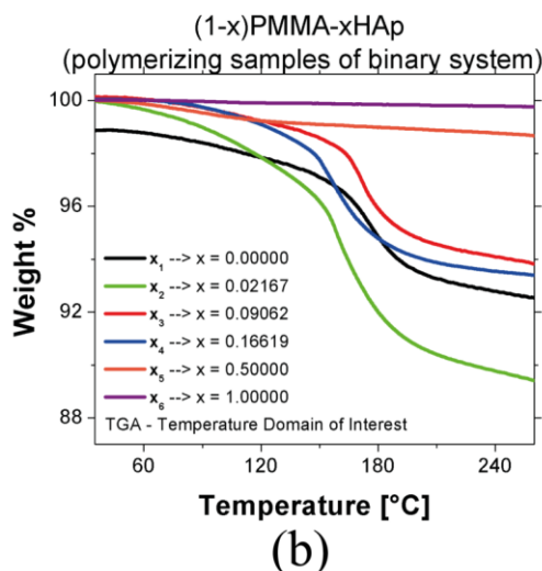
Figure 3. TGA heating profiles for x_i ( i=1-6 ) concentrations of the (1-x)PMMA-xHAp polymerizing samples to determine system's mass loss (a) among 35 – 751 °C (b) in TOI among 45 – 240 °C approximately.
