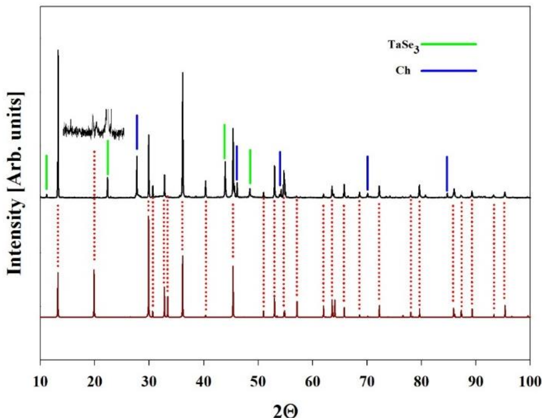
Figure 3. Comparison of the experimental diffraction pattern for sample x=0.5 for the alloy system (\text{CuGaSe}_2)_{1-x}(\text{TaSe})_x (in the top) with the calculated diffraction pattern for 2\text{H-Cu}_{0.52}\text{TaSe}_2 sample (in the bottom). The insert is an amplification of the particular region. Green ticks: \text{TaSe}_3 phase; Blue ticks: chalcopyrite \text{CuAlSe}_2 -like phase.
